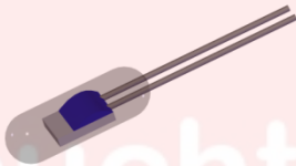
Fig. 2: Thin-layer Measuring Resistor in a glass housing (M-MG)
