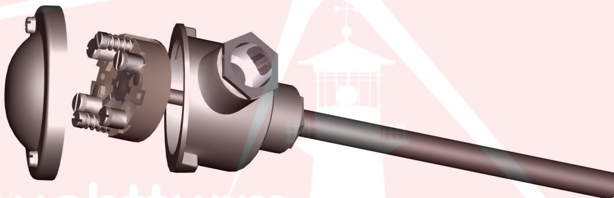
Fig. 15: LTH-B with DIN head form B, and exchangeable measuring insert in a 4-wire connection
